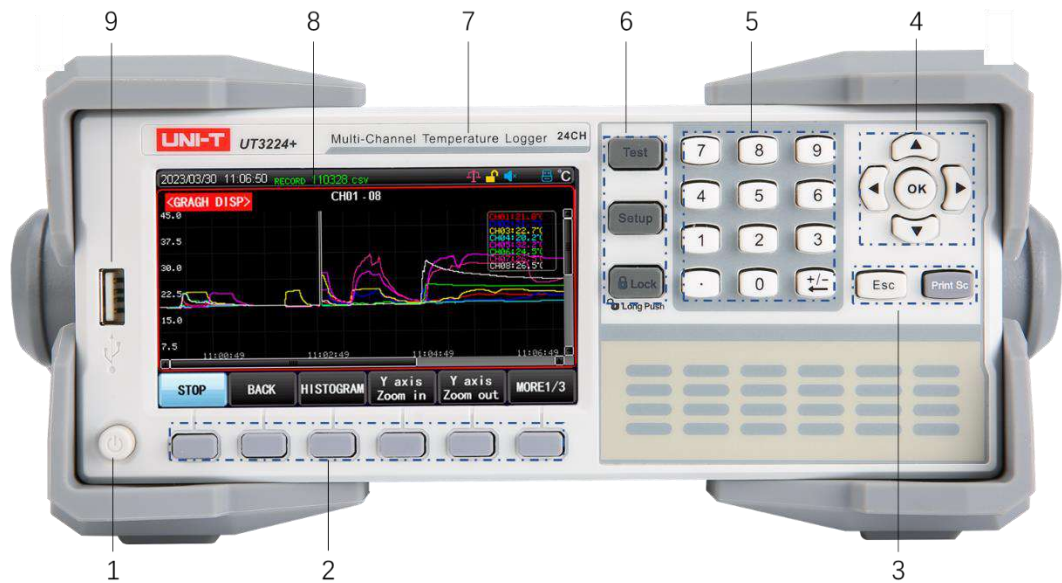
Figure 4-1 Front Panel
