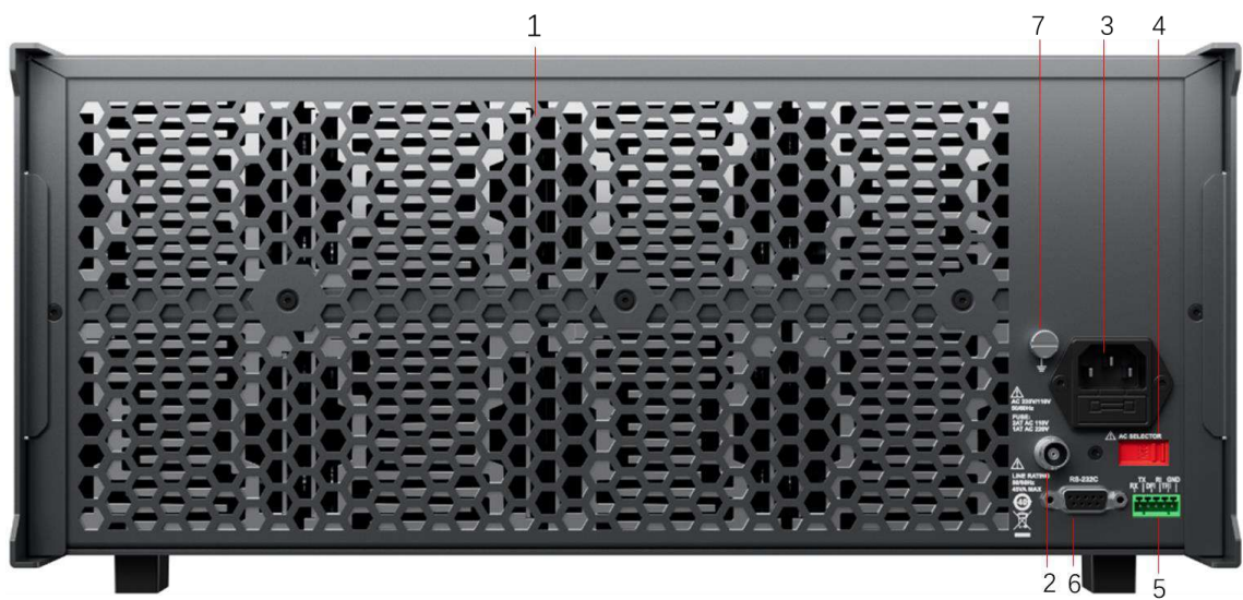
Figure 4-2 Rear Panel
