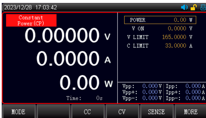
Figure 7-1-7 CP Mode
