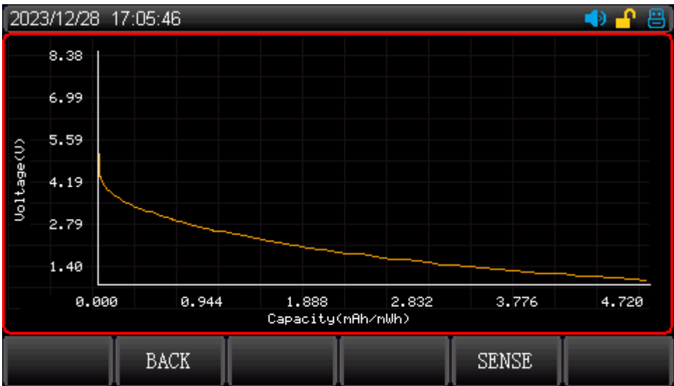
Figure 7-2-12 Charge and Discharge Curve
